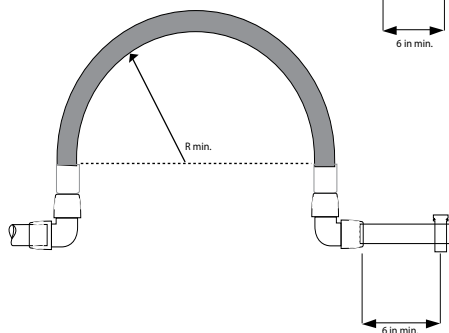
Expansion loop
